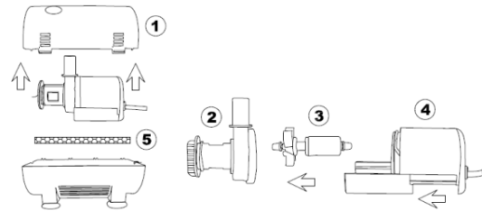
① PUMP CASE ② IMPELLER COVER ③ IMPELLER ④ PUMP ⑤ FILTER
