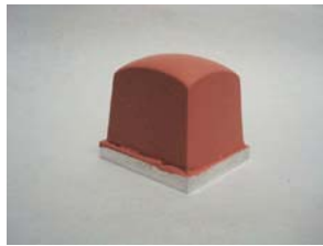
N6 - Overall Height Incl. Base Shown: 1.95 in. length at base: 1.6 in Width at base: 1.9 in Base Shown: (aluminum) .25in
