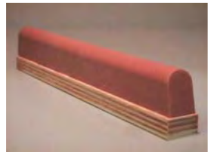
D8 - Overall Height Including Base Shown: 1 3/8 in. Overall Length of Rubber: 8 5/8 in. Overall Width of Rubber: 9/16 in. Base Shown: (wood) 8 3/4 in. x 7/8 in. x 1/2
