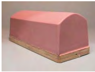
T2 - Overall Height Incl Base Shown: 3 7/8 in. Length at Base: 8 7/8 in. Length at Top: 8 1/2 in. Width at Base: 3 3/4 in. Width at Top: 3 1/2 in. Base Shown: (wood) 9 3/16 in. x 3 7/8 in. x 1/2 in
