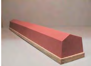
H40 - Overall Height Incl Base Shown: 2 \frac{3}{8} in. Length at Base: 18 \frac{3}{8} in. Length at Top: 17 \frac{7}{8} in. Width at Base: 2 \frac{1}{2} in. Width at Top: 2 in.
