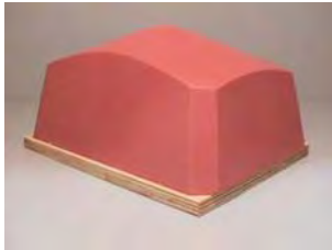
G31 - Overall Height Incl Base Shown: 4 5/8 in. Length at Base: 8 5/16 in. Length at Top: 7 1/4 in. Width at Base: 6 3/16 in. Width at Top: 5.0 in. Base Shown: (wood) 8 5/16 in. x 6 7/16 in. x 1/2 in
