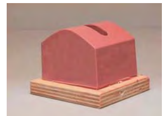
H52 - Overall Height incl Base Shown: 2 \frac{1}{8} in. Overall Length : 2.0 in. Overall Width : 2 \frac{1}{4} in. Hole in Center of Rubber measuring: 1 \frac{7}{16} in. x \frac{5}{16} in. x \frac{7}{8} in. deep Base Shown: (wood) 2 \frac{5}{8} in. x 2 \frac{3}{8} in. x \frac{3}{8} in
