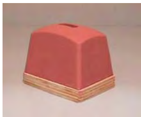
T25 - Overall Height incl Base Shown: 2 1/2 in. Length at Base: 2 13/16 in. Length at Top: 2 1/2 in. Width at Base: 2 1/16 in. Width at Top: 1 5/8 in. Hole in Center measuring: 15/16 in. x 3/8 in. x 1/2 in. deep Base Shown: (wood) 3.0 in. x 2 1/4 in. x 1/2 in
