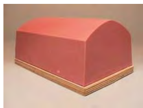
H45 - Overall Height Incl Base Shown: 3 \frac{5}{8} in. Length at Base: 7.0 in. Length at Top: 6 \frac{3}{4} in. Width at Base: 4 \frac{3}{4} in. Width at Top: 4 \frac{5}{16} in.
