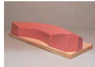
H94 - Overall Height Incl Base Shown: 2 1/8 in. Overall Length: 10 9/16 in. Overall Width: 2 13/16 in. Base Shown: (wood) 10 11/16 in. x 3 7/8 in. x 1/2 in
