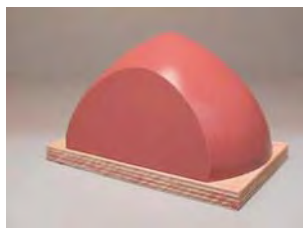
G23 - Overall Height Including Base Shown: 3 1/4 in. Overall Length : 5 3/8 in. Width at Base: 3 5/8 in. Width at Top 2 3/4 in. Base Shown: (wood) 5 7/16 in. x 3 5/8 in. x 1/2 in
