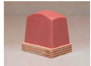
H47 - Overall Height incl Base Shown: 2 \frac{1}{4} in. Length at Base: 2 \frac{1}{16} in. Length at Top: 1 \frac{7}{8} in. Width at Base: 1 \frac{1}{4} in. Width at Top: 1 \frac{1}{16} in. Base Shown: (wood) 2 \frac{5}{16} in. x 1 \frac{9}{16} in. x \frac{3}{8} in
