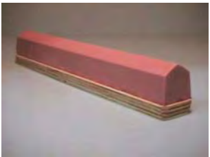
D43 - Overall Height Incl. Base Shown: 15/8 in. Length at Base: 13 7/8 in. Length at Top: 13 3/4 in. Width at Base: 1 1/8 in. Width at Top: 1.0 in.
