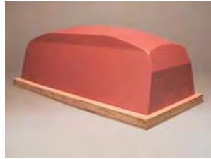
H75 - Overall Height Incl Base Shown: 5 5/8 in. Length at Base: 14 1/16 in. Length at Top: 12 3/4 in. Width at Base: 5 3/4 in. Width at Top: 4 1/8 in. Base Shown: (wood) 14 7/8 x 6 3/4 in. x 1/2 in
