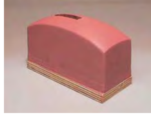
H16 - Overall Height incl Base Shown: 3.0 in. Length at Base: 4 3/4 in. Length at Top: 4 1/2 in. Width at Base: 2 1/4 in. Width at Top: 1 7/8 in. Hole in Center of Rubber measuring: 1 9/16 in. x 3/8 in. x 1 5/8 in. deep Base Shown: (wood) 4 3/4 in. x 2 1/4 in. x 1/2 in
