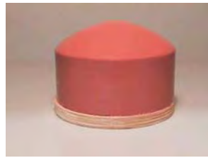
R18 - Overall Height Including Base Shown: 3 7/16 in. Overall Diameter of Rubber: 4 3/8 in. Base Shown: (wood) 4 15/16 in. d. x 1/2 in
