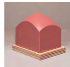
G22 - Overall Height Incl Base Shown: 3 1/4 in. Length at Base: 3 3/16 in. Length at Top: 3.0 in. Width at Base: 2 7/16 in. Width at Top: 2 5/16 in. Base Shown: (wood) 3 5/8 in. x 2 7/8 in. x 1/2 in
