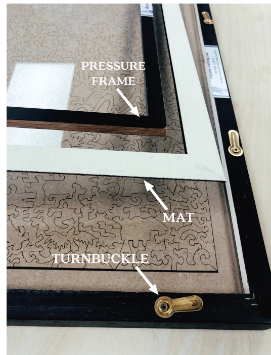
Rear detail
