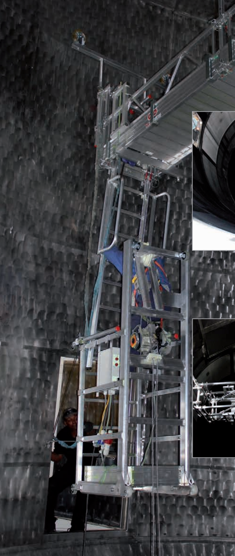
Inspection platform for silo's, tanks and spray dryers
