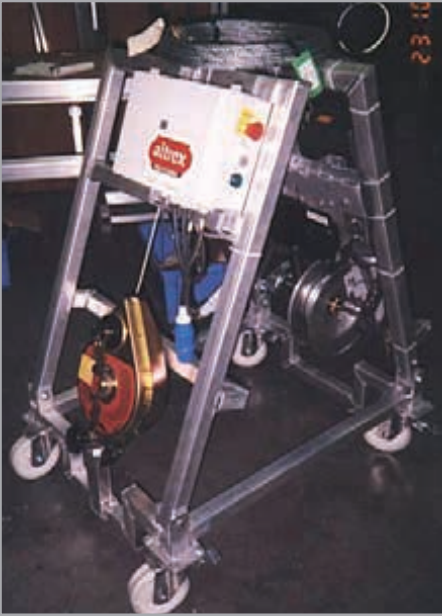
Mobile carrying console silo-descent system
