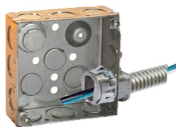
Snap fitting into box.
