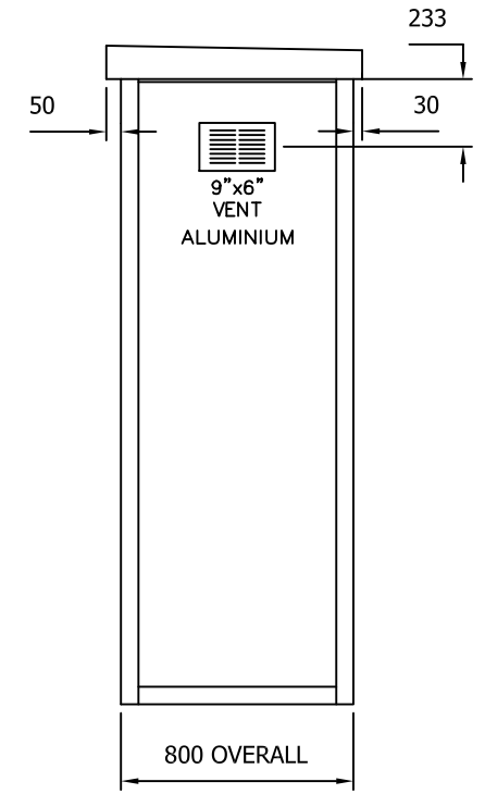
ELEVATION WALL D
