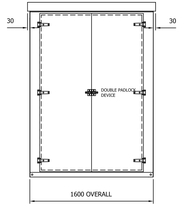
ELEVATION WALL A
