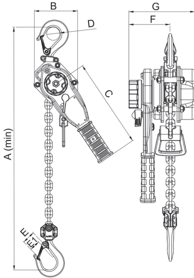
Lever hoist PREMIUM PRO 800 kg - 3200 kg
