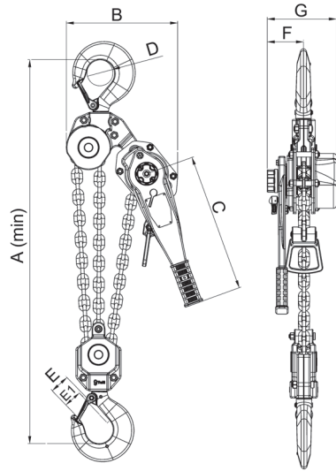
Lever hoist PREMIUM PRO 9t
