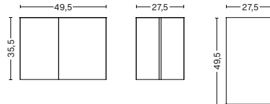
SLIT TABLE OBLONG LENGTH 49,5 CM | 19.49" WIDTH 27,5 CM | 10.83" HEIGHT 35,5 CM | 13.98"
