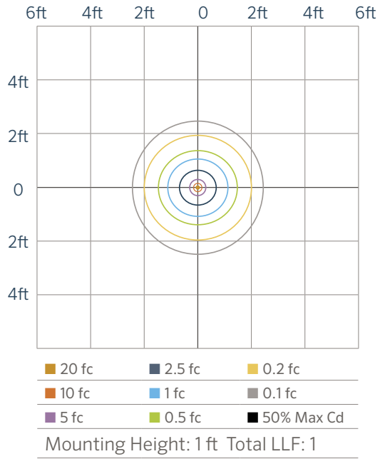
DL LED 10W ISOFOOTCANDLE PLOT
