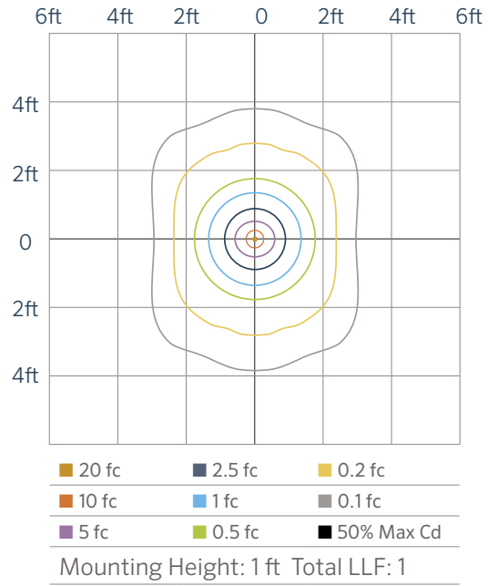
DL LED 20W ISOFOOTCANDLE PLOT
