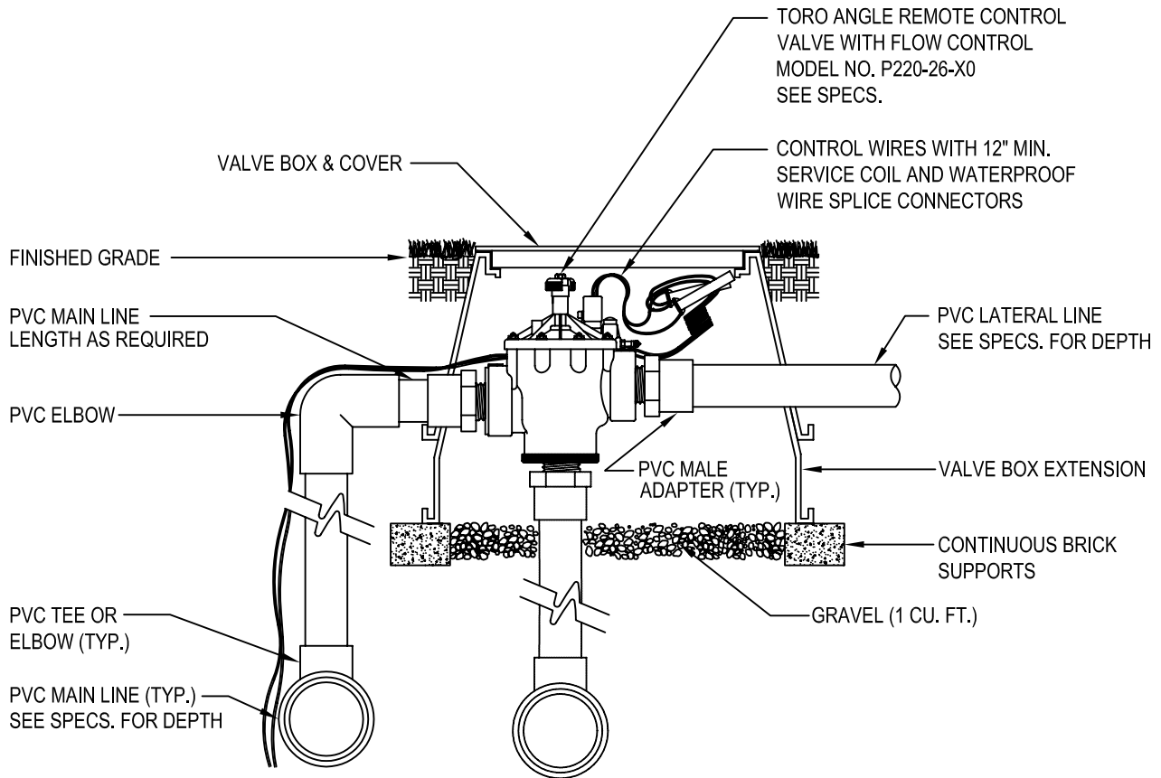
SECTION/ELEVATION NOT TO SCALE
