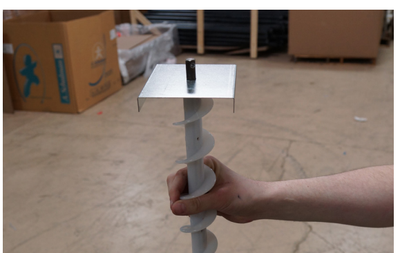
Step 8: Place spinner on top of auger.
