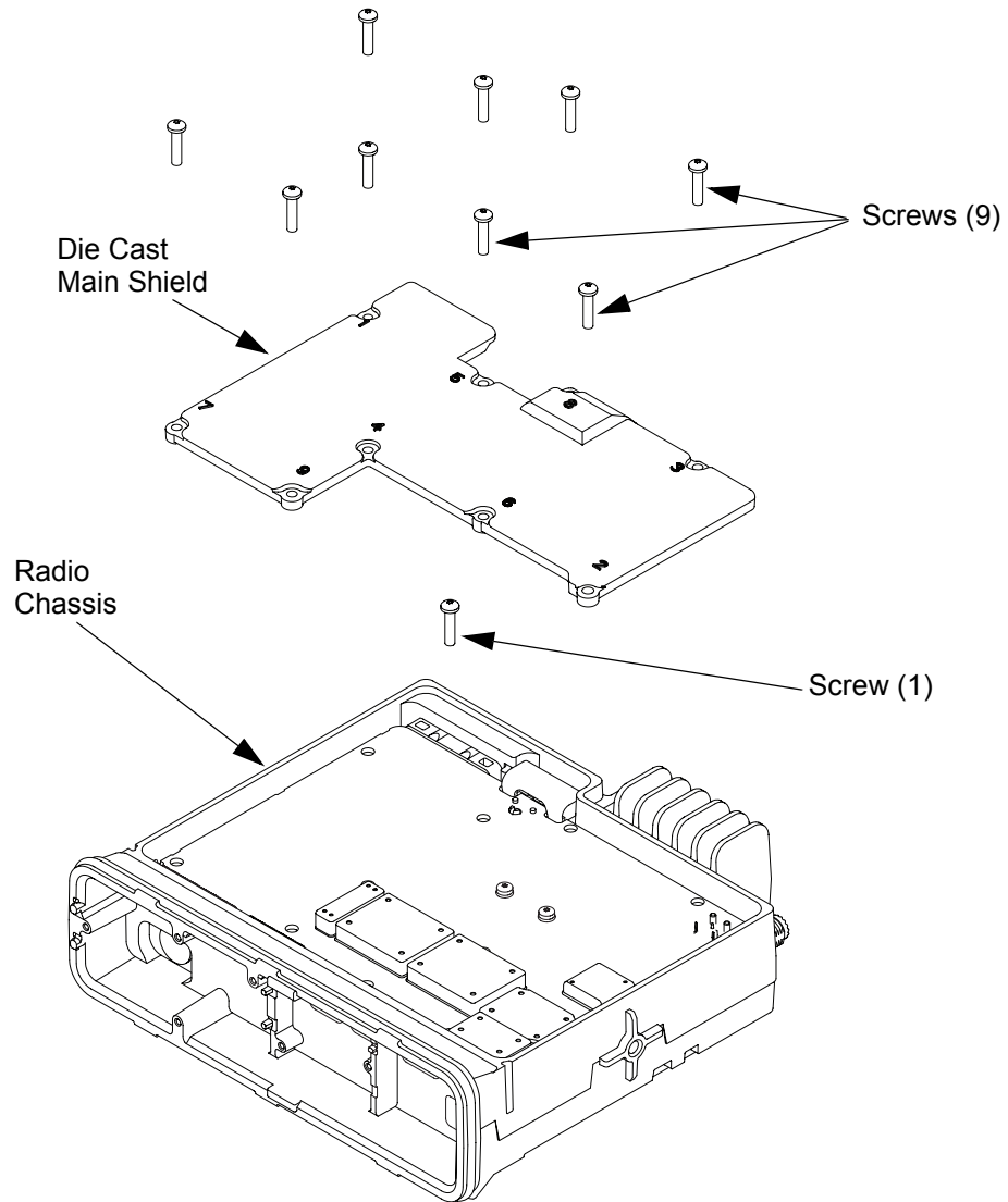
Figure 5-10 Die Cast Main Shield Removal
