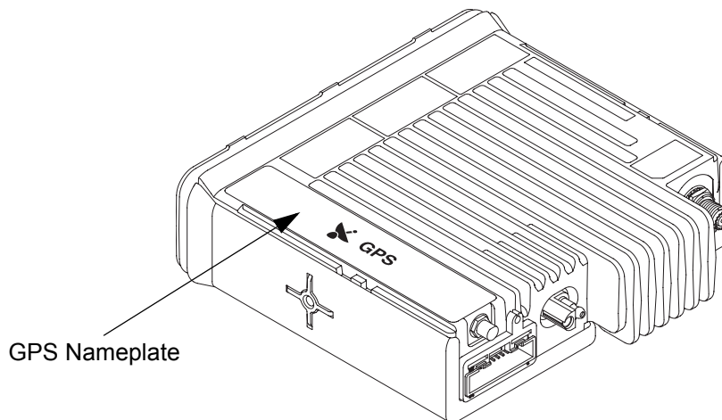
Figure 5-5 GPS Nameplate Removal
