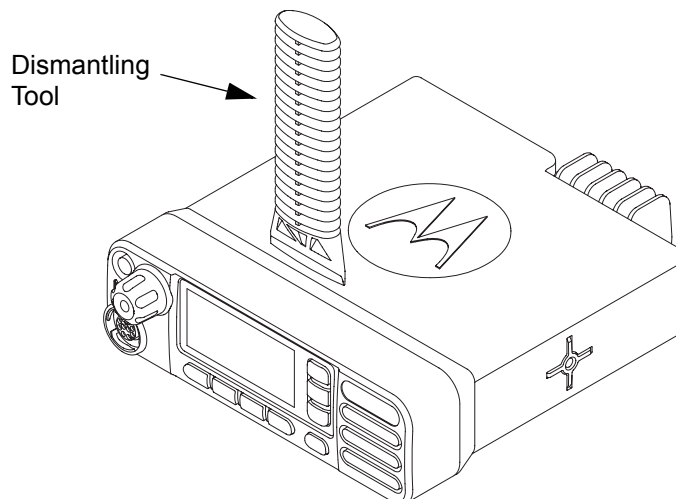
Figure 5-1 Typical Control Head Removal
