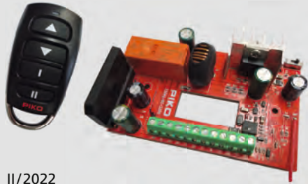
35042 R/C Loco Receiver 5A, Pure DC w/Remote
