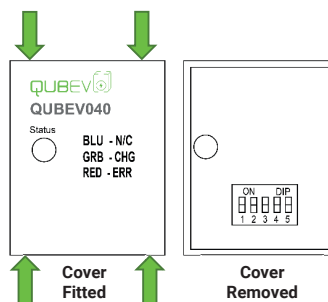
Figure 5 Charge Control Unit
