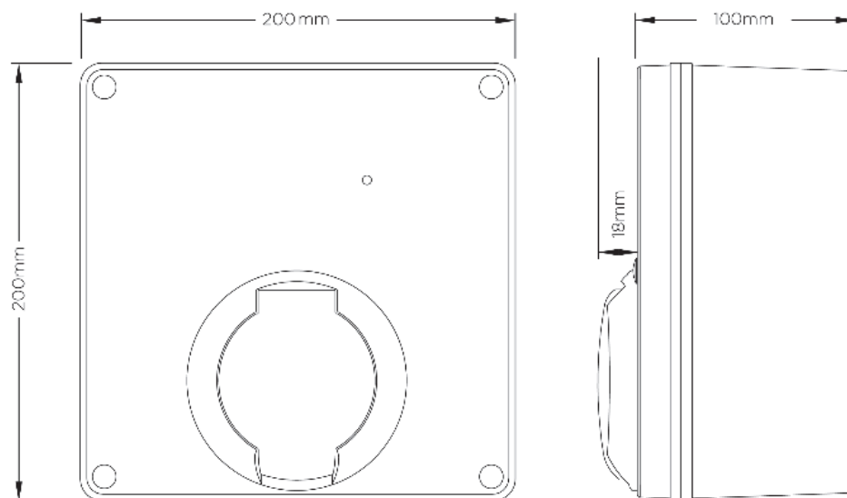
Figure 2 EVON0080 3-Phase Model
