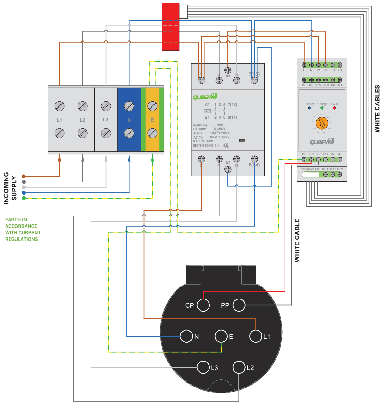
Figure 7 EVON0080 - Schematic Diagram (3-Phase Model)
