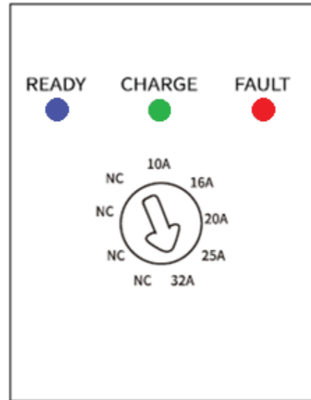
Figure 8 Charge Control Unit
