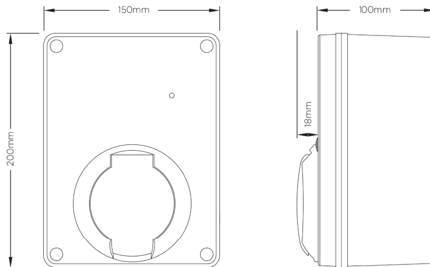
Figure 1 EVON0040 1-Phase Model
