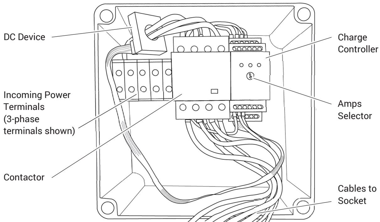
Figure 3 General Arrangement
