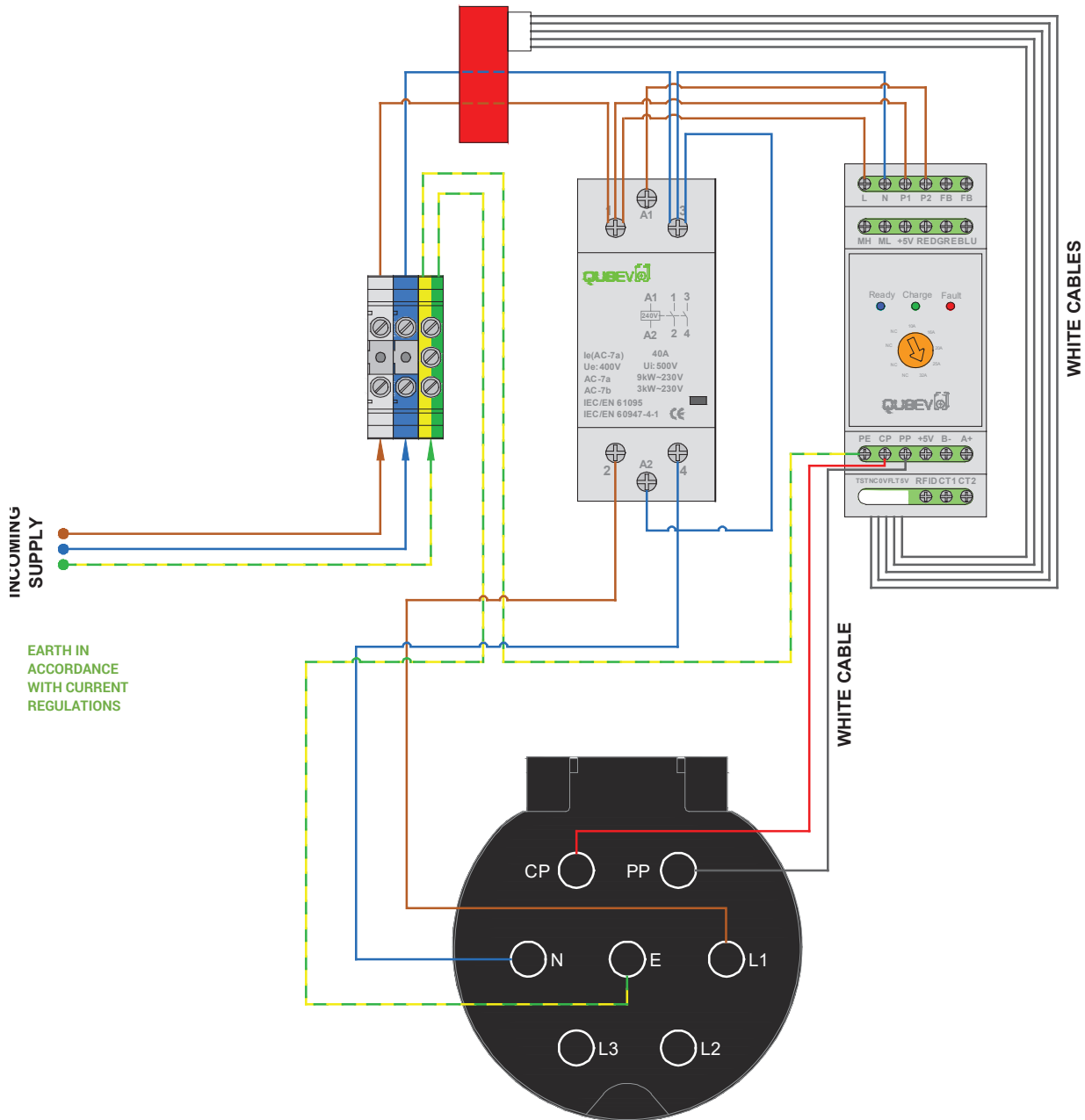
Figure 6 EVON0040 - Schematic Diagram (1-Phase Model)
