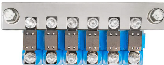
Stacked fuse holders with 6-position high current bus bar (copper 40 x 5 mm)
