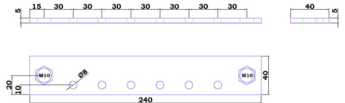
CIP100400070 = Busbar to connect 6 CIP100200100
