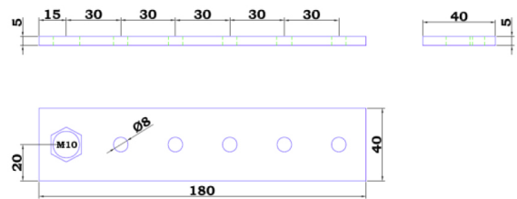
CIP100400060 = Busbar to connect 5 CIP100200100
