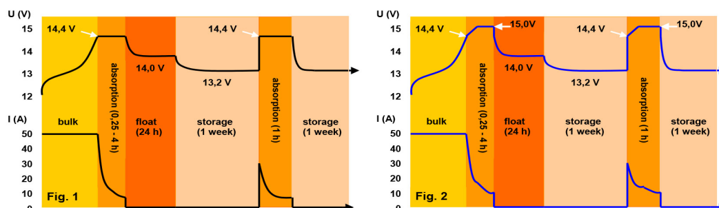
Charge curves: up to the gassing voltage (fig.1), and exceeding the gassing voltage (fig.2)
