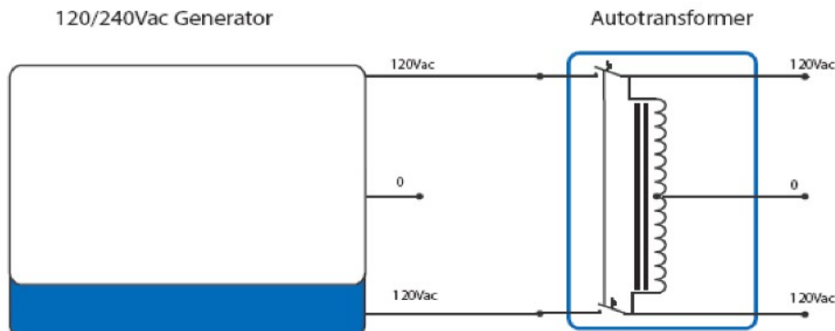
Stacked inverter balancing (Ground relay of autotransformer should be used)
