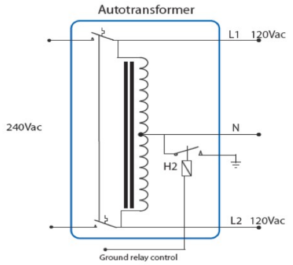
Autotransformer: schematic diagram
