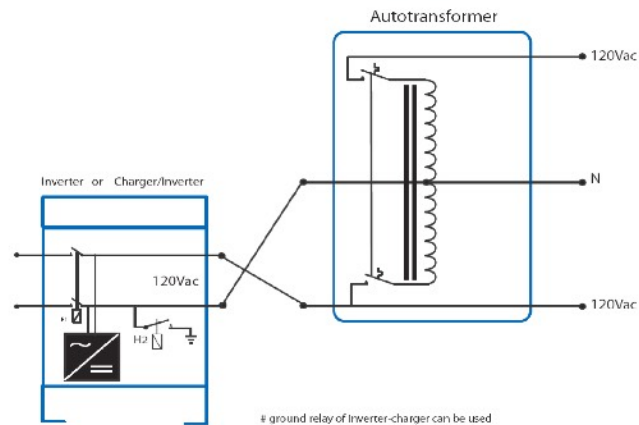
Split phase: 120VAC to 120/240VAC (Internal ground relay of inverter/charger may be used)
