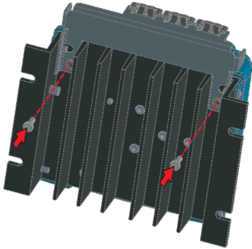
STEP 1: Mount the 'steel base' to the MPPT before installation to the wall.
