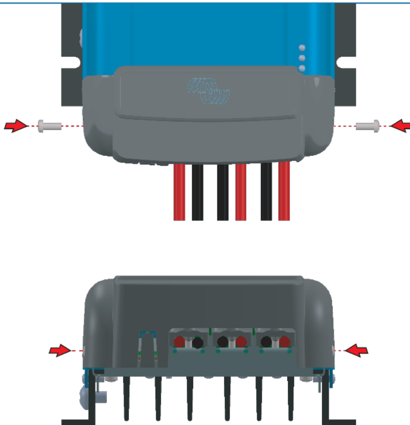
STEP 3: Place the WireBox cover and fasten with two screws.
