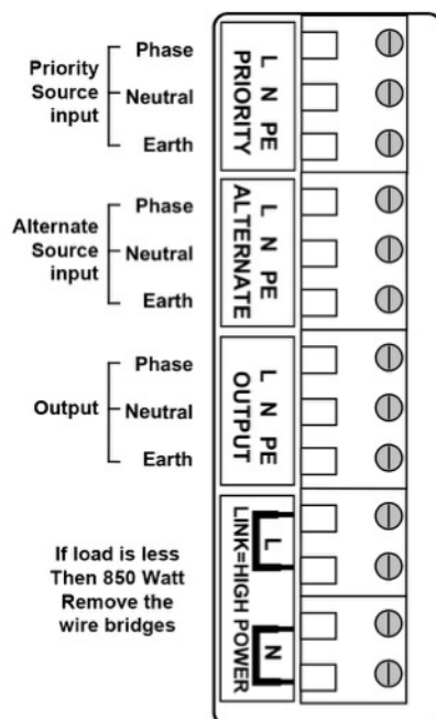
Wiring diagram
