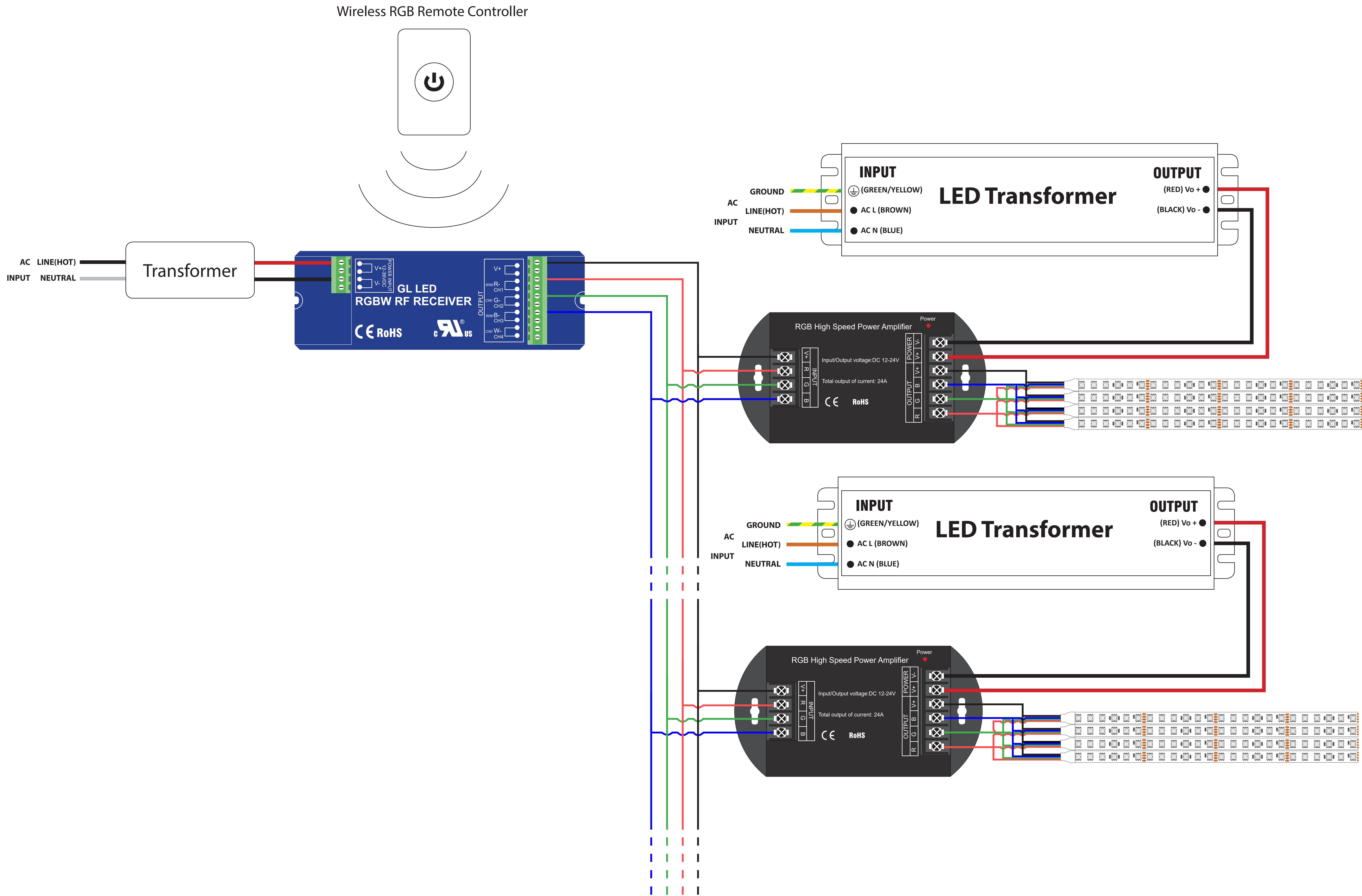
Wiring diagram - RGB Color Changing Wireless Controller with BLK RGB Amplifier
