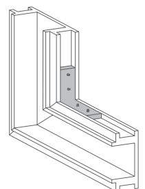
AL L-Shape Corner Connector - Vertical
