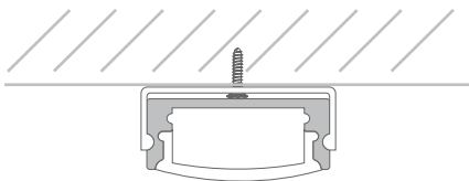
Surface mounting with Mounting Clips
