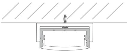
Surface mounting with Mounting Clips
