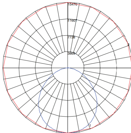
Maximum Candela = 15476.2 Located At Horizontal Angle = 90, Vertical Angle = 2 # 1 - Vertical Plane Through Horizontal Angles (90 - 270) (Through Max. Cd.) # 2 - Horizontal Cone Through Vertical Angle (2) (Through Max. Cd.)
