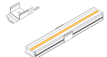
Channel Mounting Clip GL-LV-MCHC
