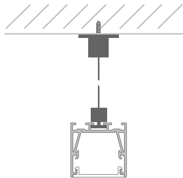
Suspended Mounting
