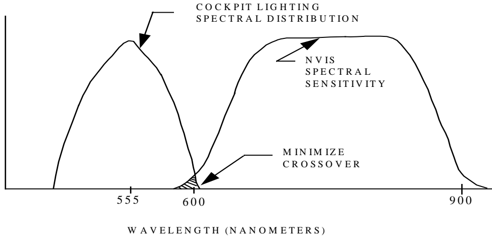
FIGURE C-2. Conceptual diagram of the spectral distribution of NVIS-compatible lighting.
