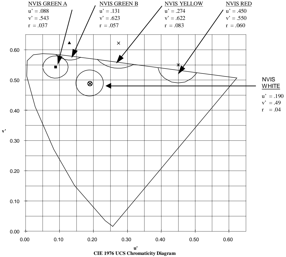
FIGURE 2. NVIS lighting color limits.
