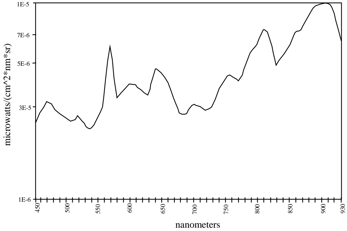
FIGURE C-9. Spectral distribution of starlight.
