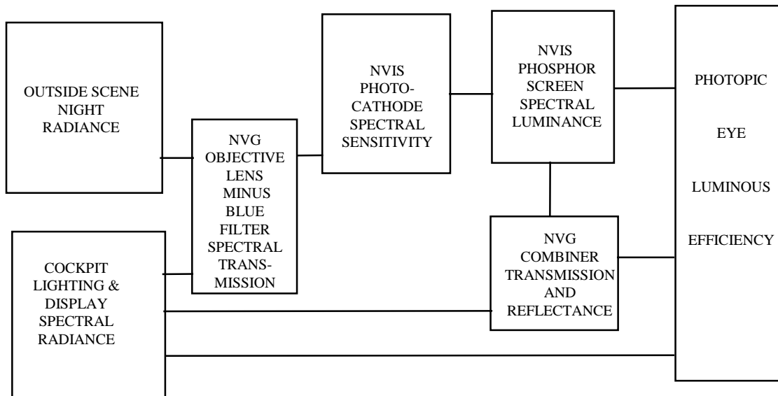
FIGURE C-3. NVIS interfaces.
