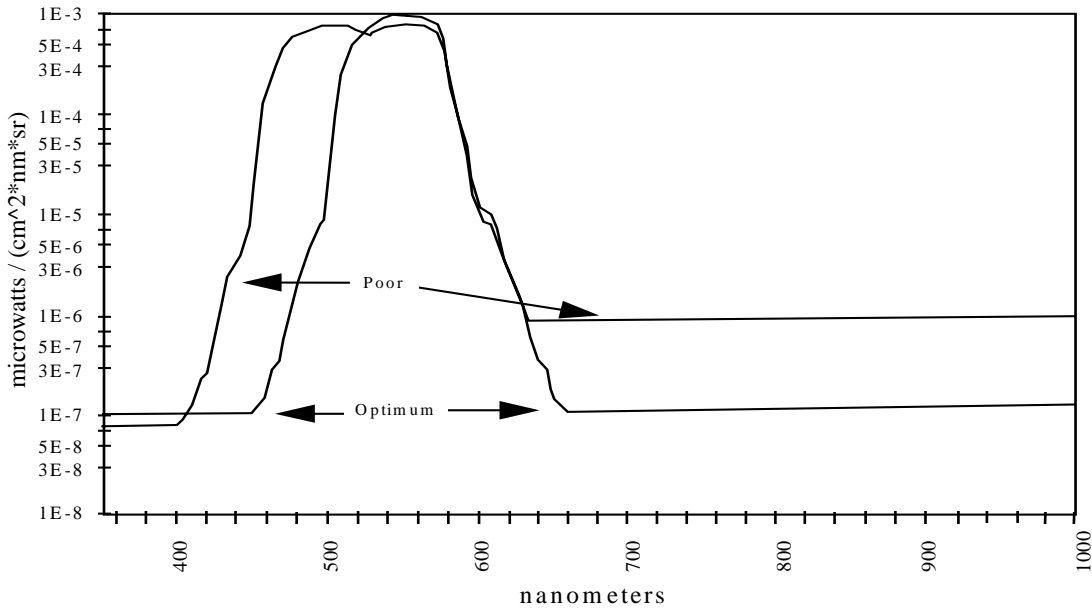
FIGURE C-7. “Optimum” and “poor” theoretical spectral distributions.
