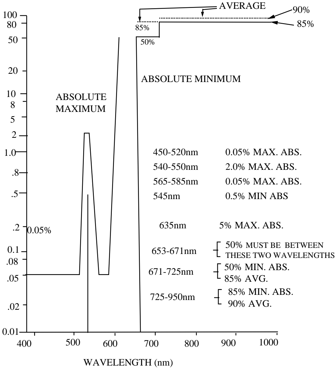
FIGURE C-6. Spectral transmission requirements for a Class C NVIS objective lens.
