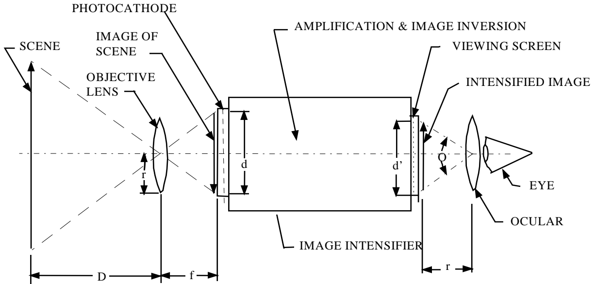
FIGURE C-1. Diagram of an image intensifier.
