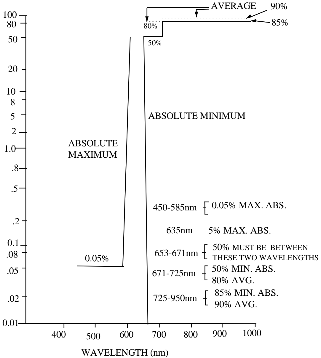
FIGURE C-5. Spectral transmission requirements for a Class B NVIS objective lens.
