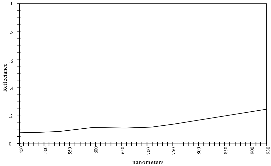
FIGURE C-10. Spectral reflectivity of tree bark.
