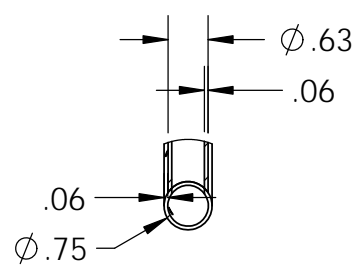
DETAIL D SCALE 1 : 3
