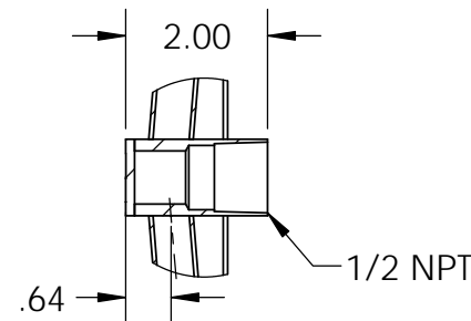
DETAIL C SCALE 1 : 3
