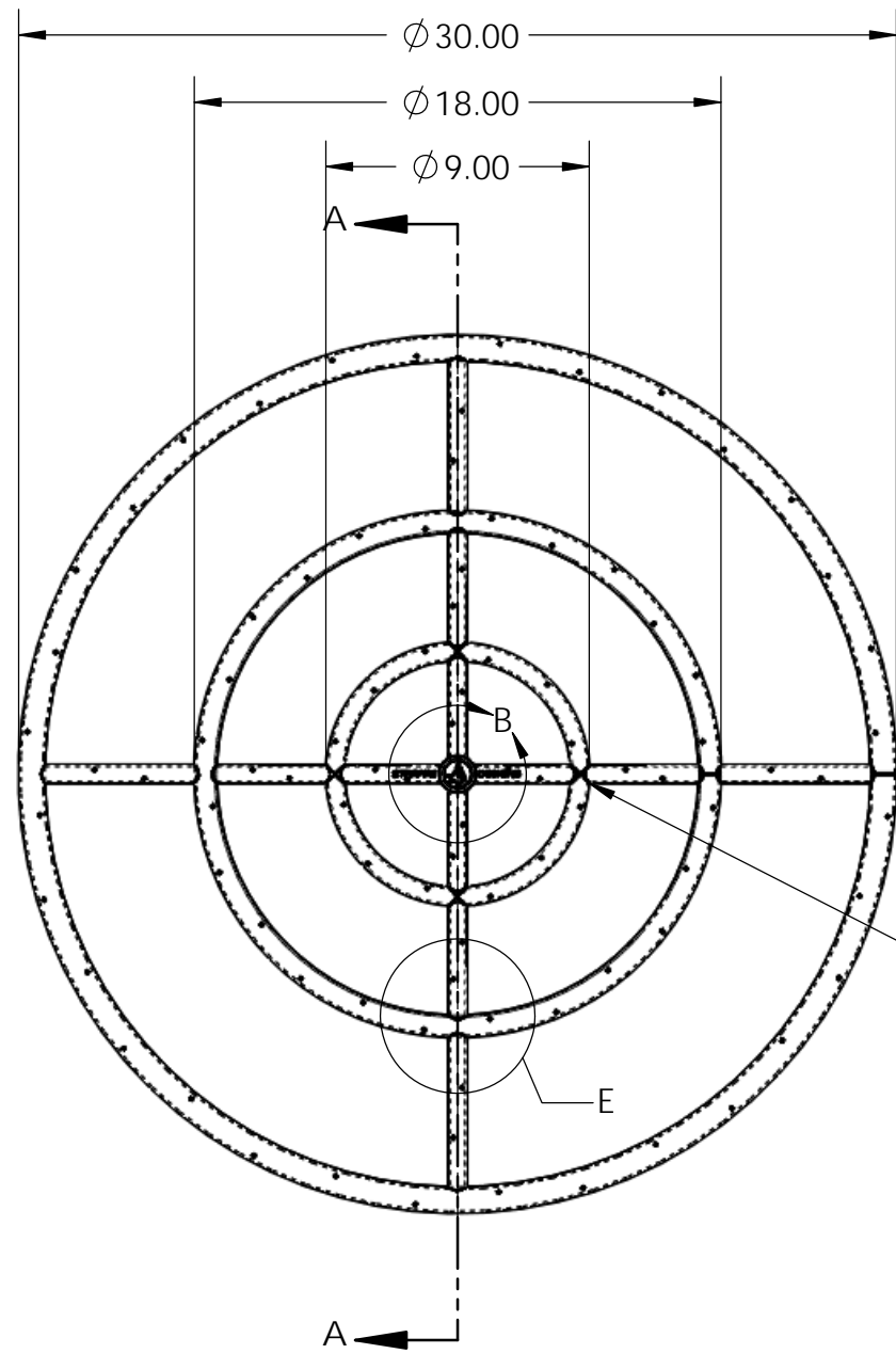
TOP VIEW
