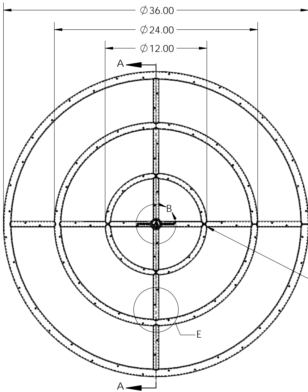
TOP VIEW
