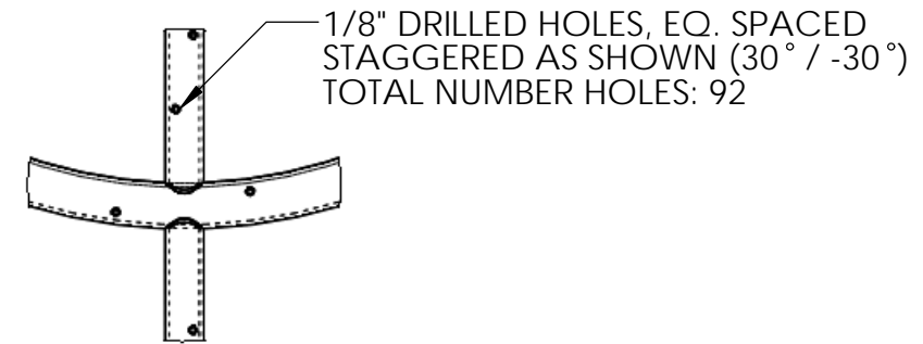
DETAIL E SCALE 2 : 7
