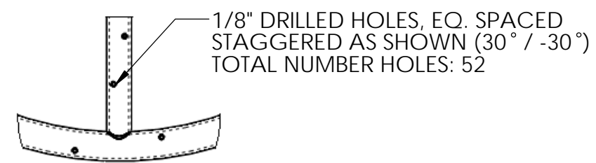
DETAIL E SCALE 2 : 7
