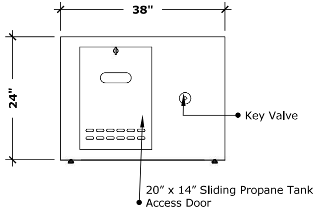
RIGHT VIEW
