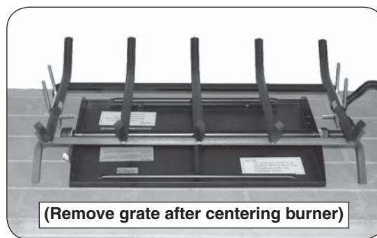
Fig. 10-2 Position grate
