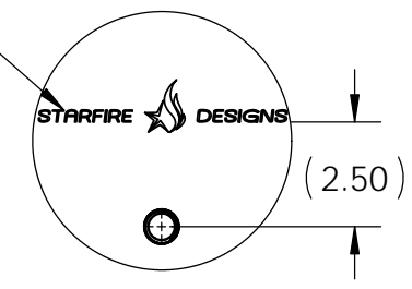
DETAIL C SCALE 1 : 5
