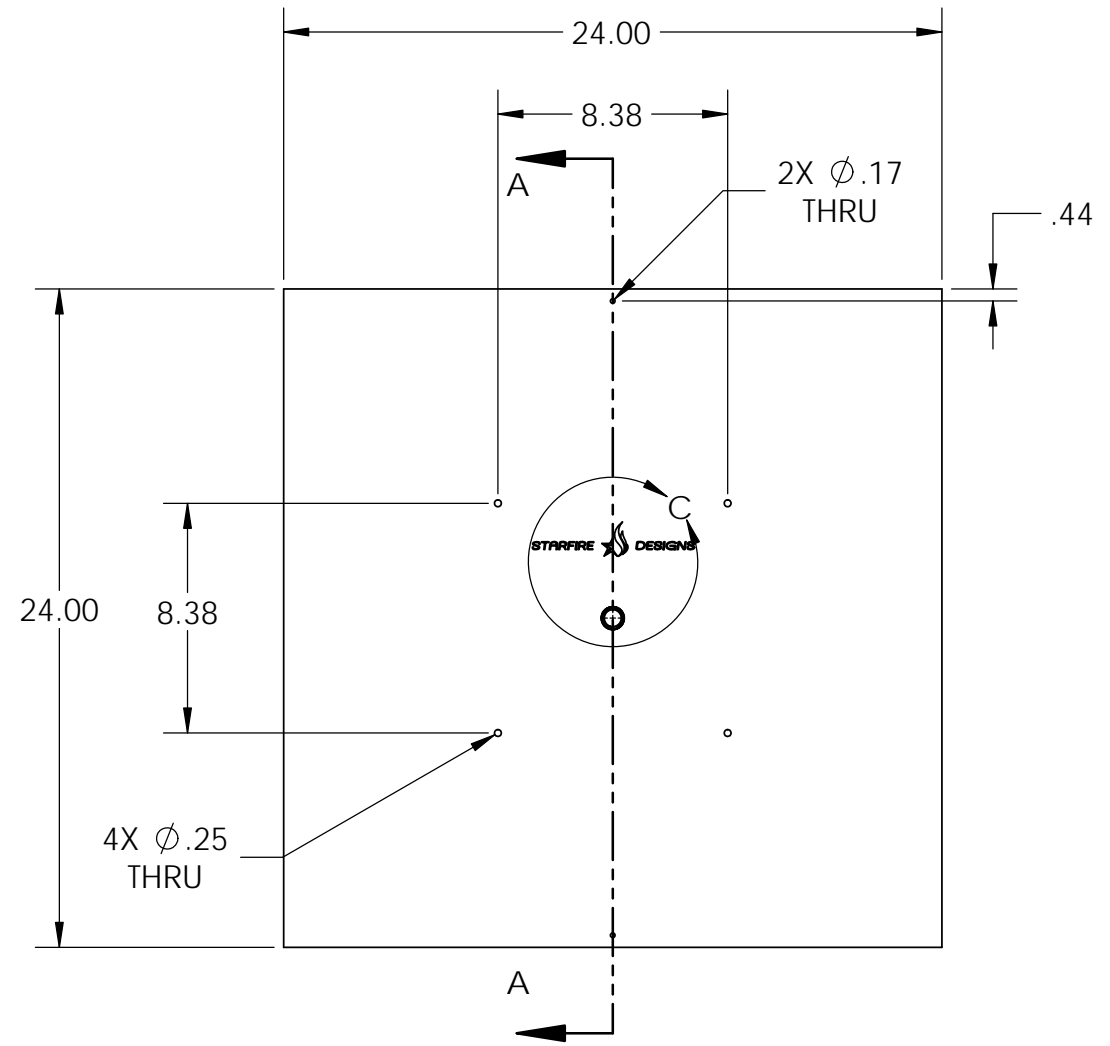
TOP VIEW
