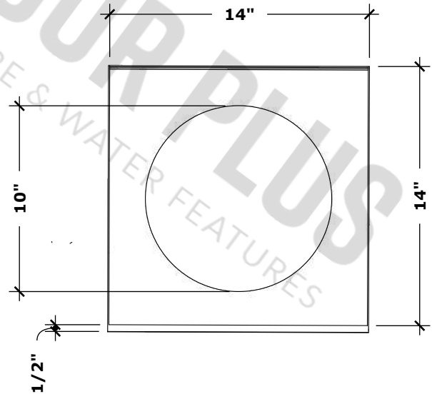
UNDERSIDE VIEW
