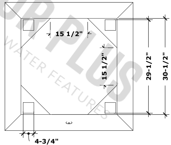
UNDERSIDE VIEW
