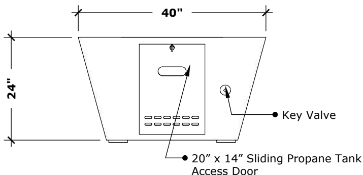
RIGHT VIEW
