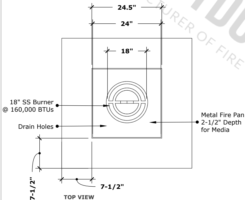
TOP VIEW
