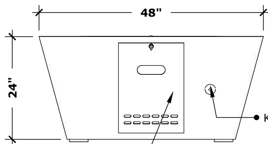
RIGHT VIEW
