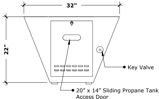
RIGHT VIEW
