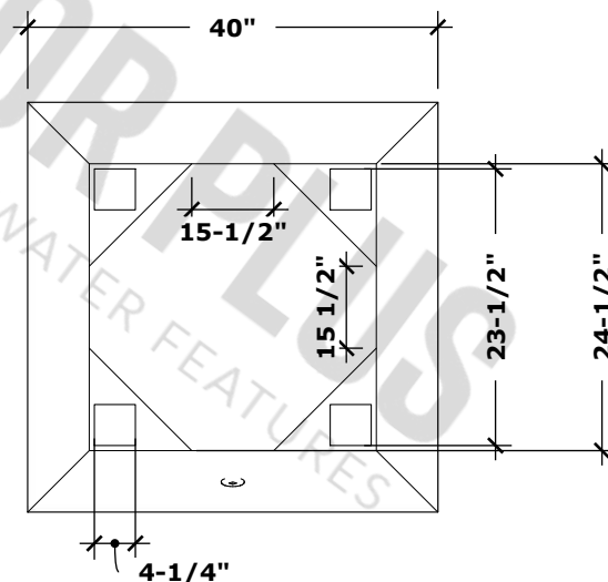
UNDERSIDE VIEW
