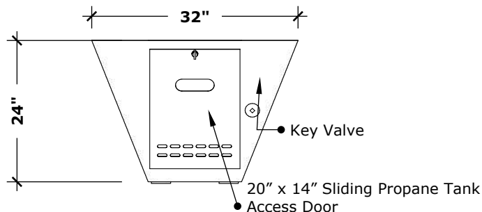
RIGHT VIEW
