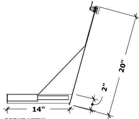
RIGHT VIEW
