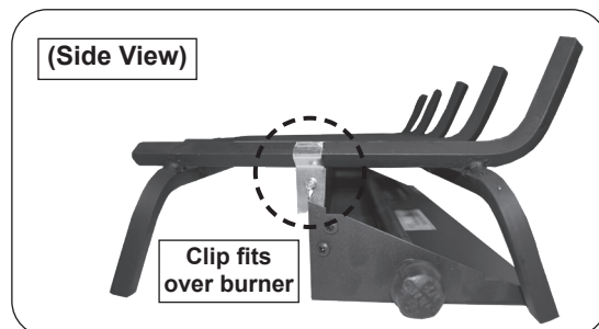
Fig. 13-3 Grate placement detail
