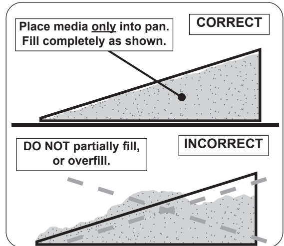
Fig. 14-2 Correct/Incorrect media placement (sand or vermiculite)
