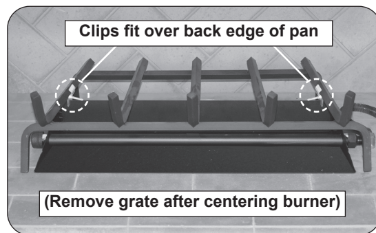
Fig. 13-2 Position grate
