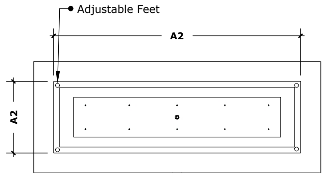
UNDERSIDE VIEW
