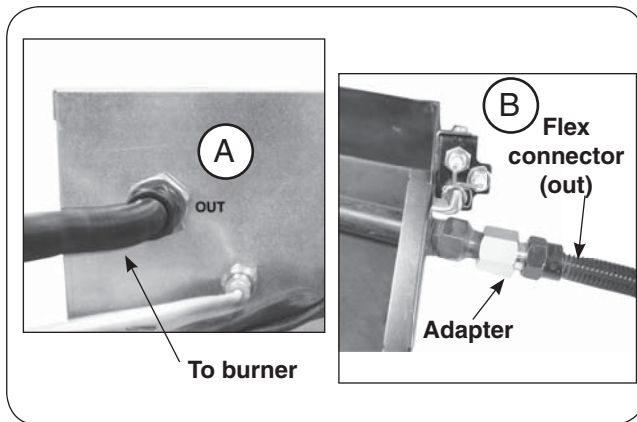
Fig. 8-1 Connect to burner
