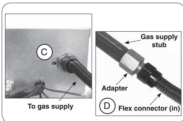
Fig. 8-2 Connect to gas supply
