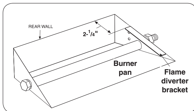
Fig. 7-1 Install diverter bracket (if applicable)
