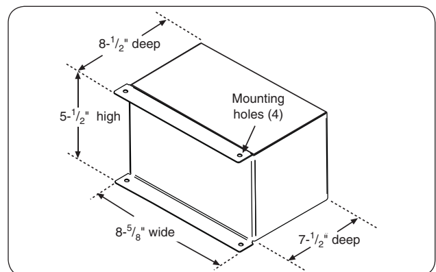
Fig. 6-2 Valve housing cutout dimensions
