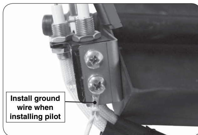
Fig. 7-4 Ground wire to bracket detail
