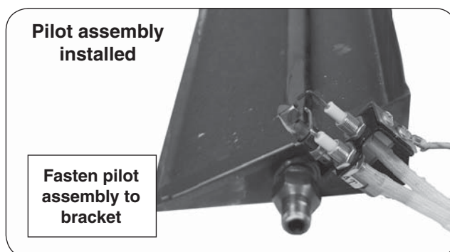
Fig. 7-3 Install pilot assembly
