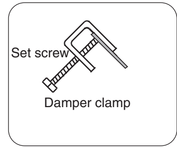
Fig. 9-1 Damper clamp detail
