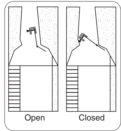
Fig. 9-2 Damper open / closed
