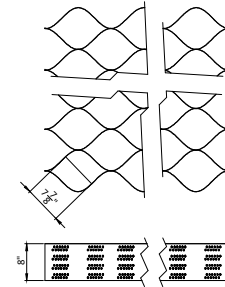
GeoCell (art.8720)
