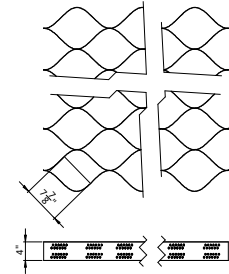
GeoCell (art.8710)
