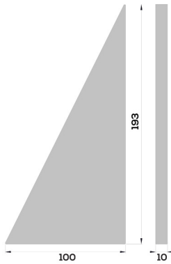
Line Drawing (mm) Variation in size can be expected
