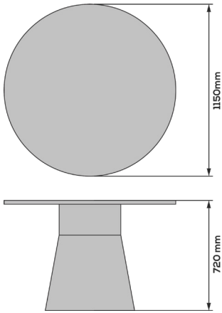
Line Drawing (mm)
