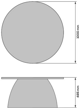
Line Drawing (mm)
