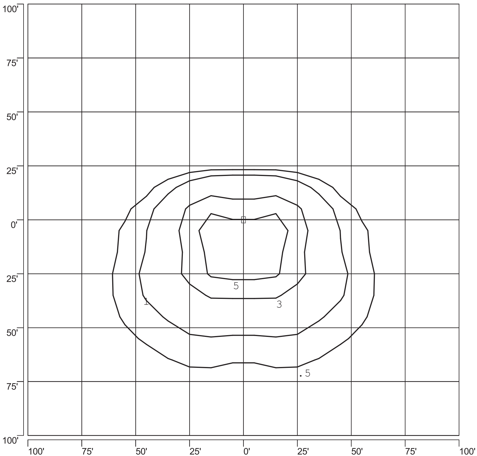
ISOFOOTCANDLE PLOT: WBVBL3-PS 400W PSMH FORWARD THROW 25' AFG - 0 DEGREE TILT
