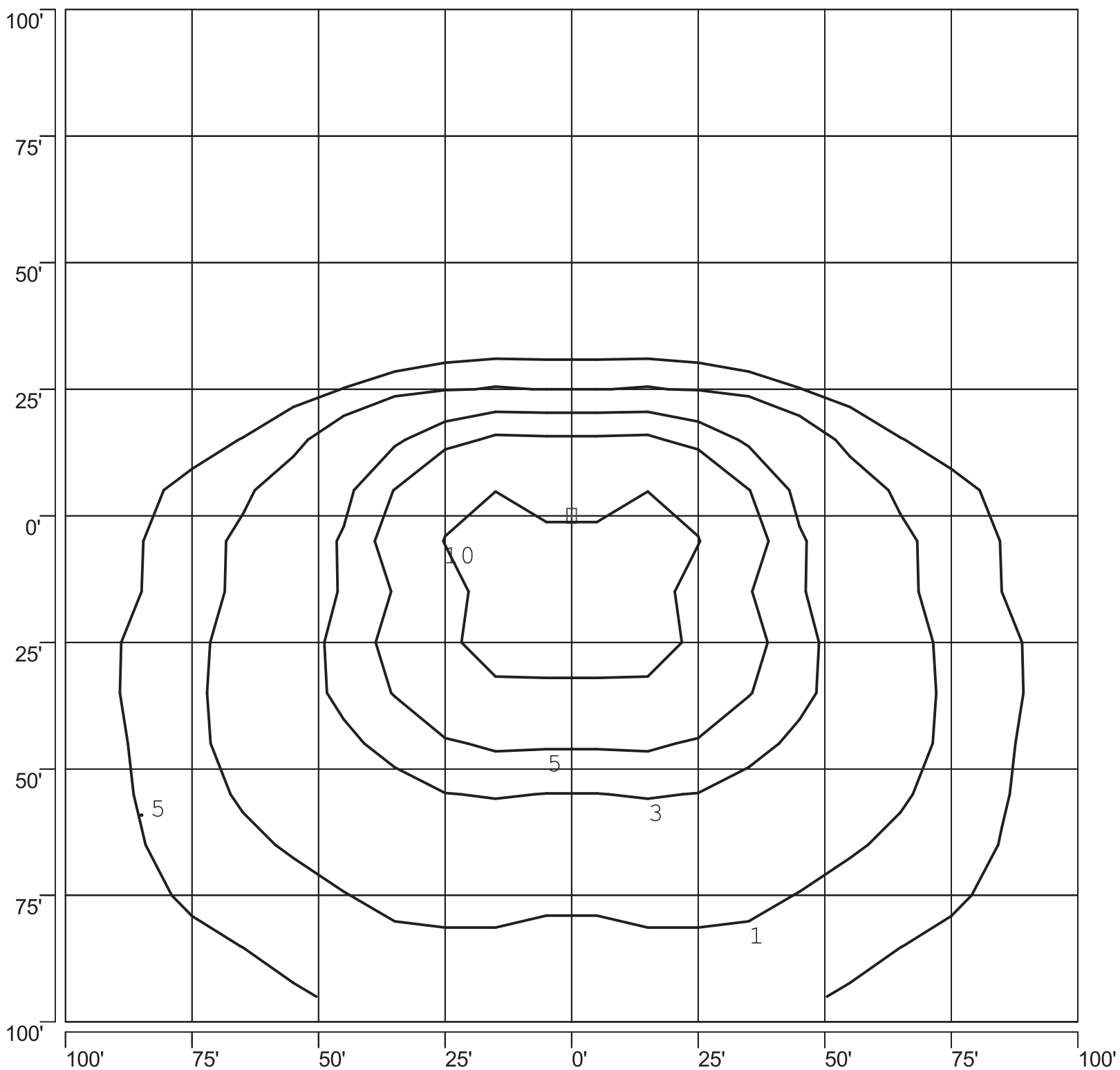
ISOFOOTCANDLE PLOT: WBVBL1 1000W MH FORWARD THROW 30' AFG - 0 DEGREE TILT
