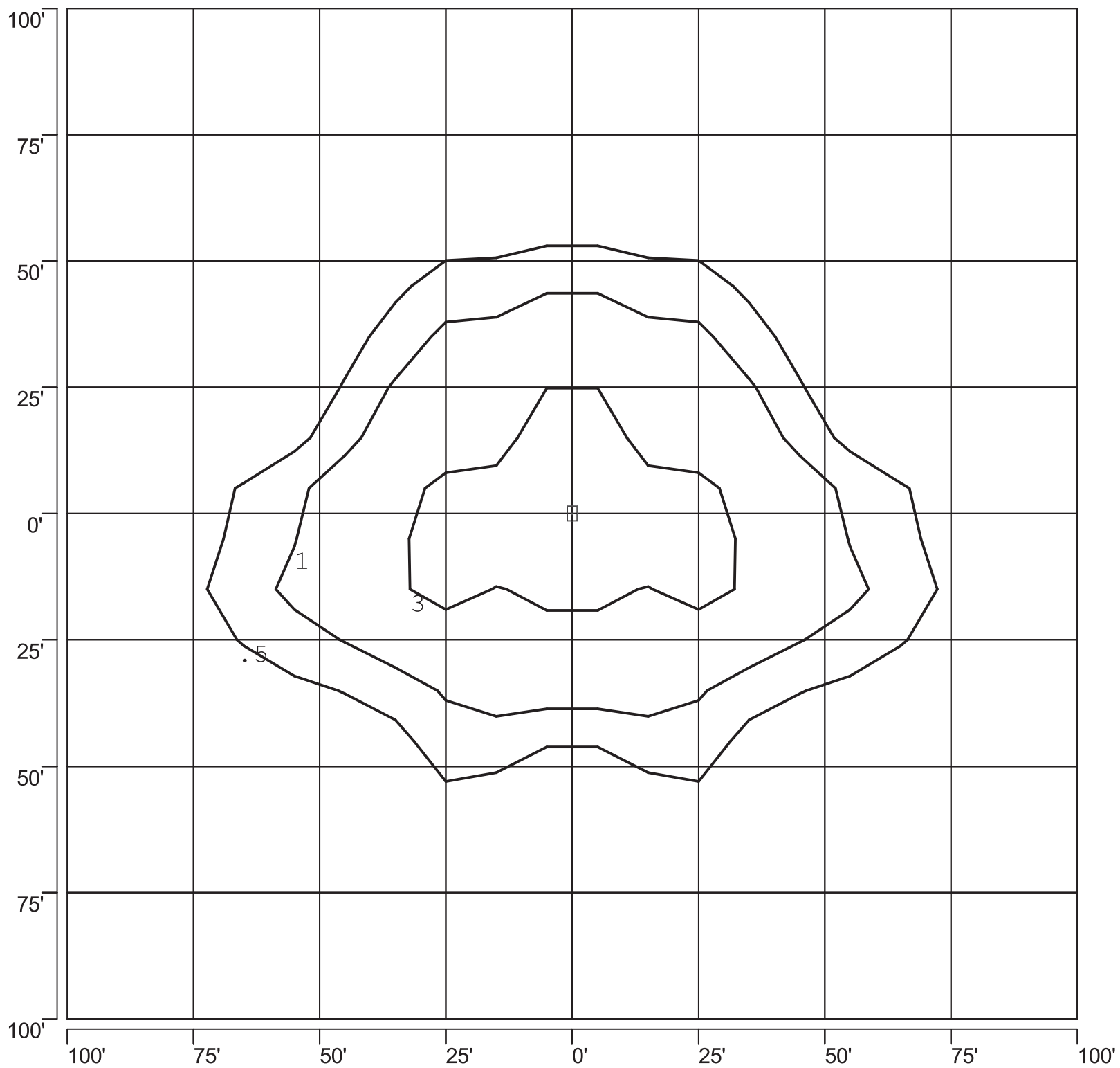
ISOFOOTCANDLE PLOT: VBMAK3B_2-PS 400W PSMH TYPE 2 25' AFG - 0 DEGREE TILT
