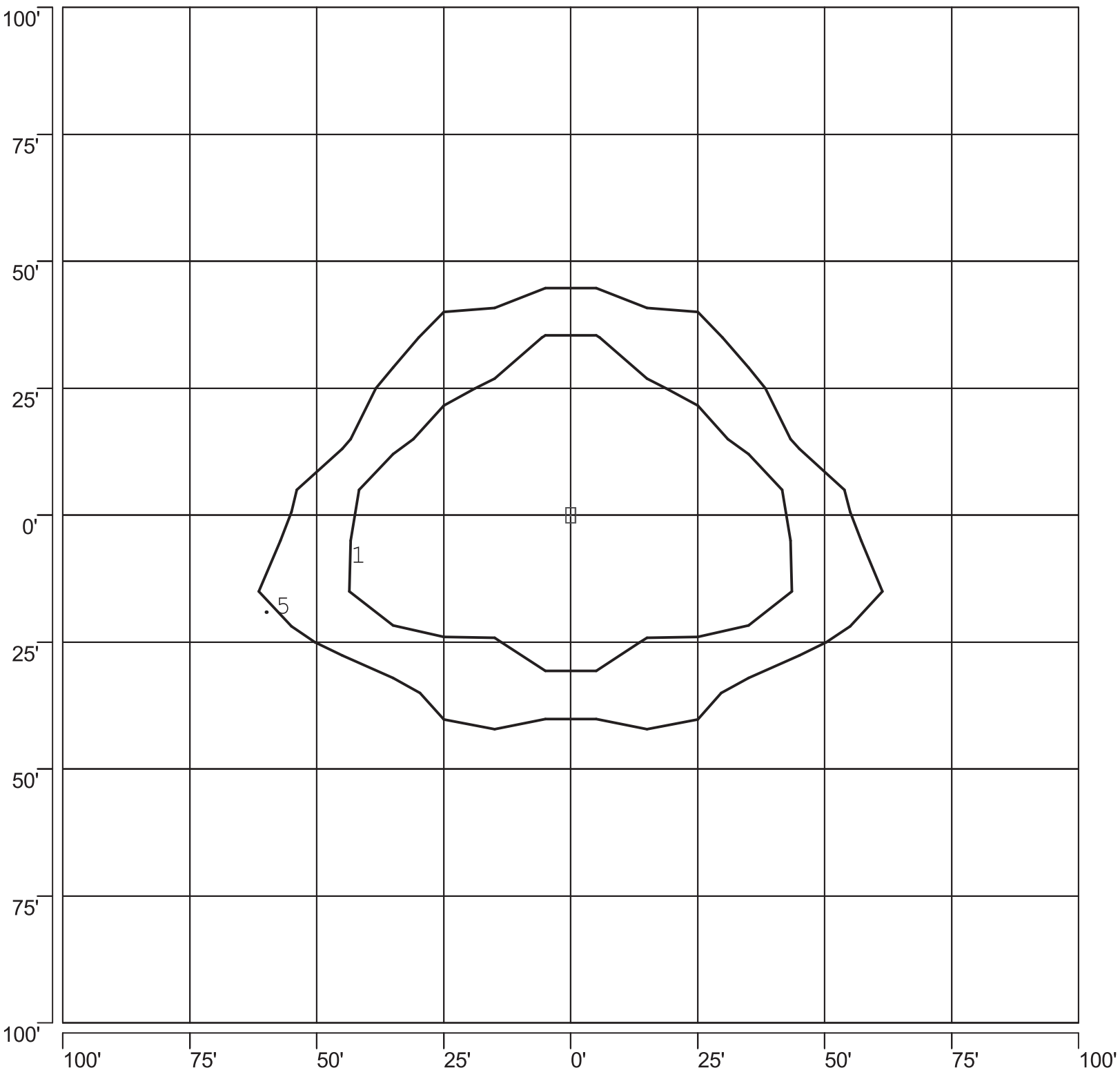
ISOFOOTCANDLE PLOT: VBMAK1B_2-PS 250W PSMH TYPE 2 25' AFG - 0 DEGREE TILT
