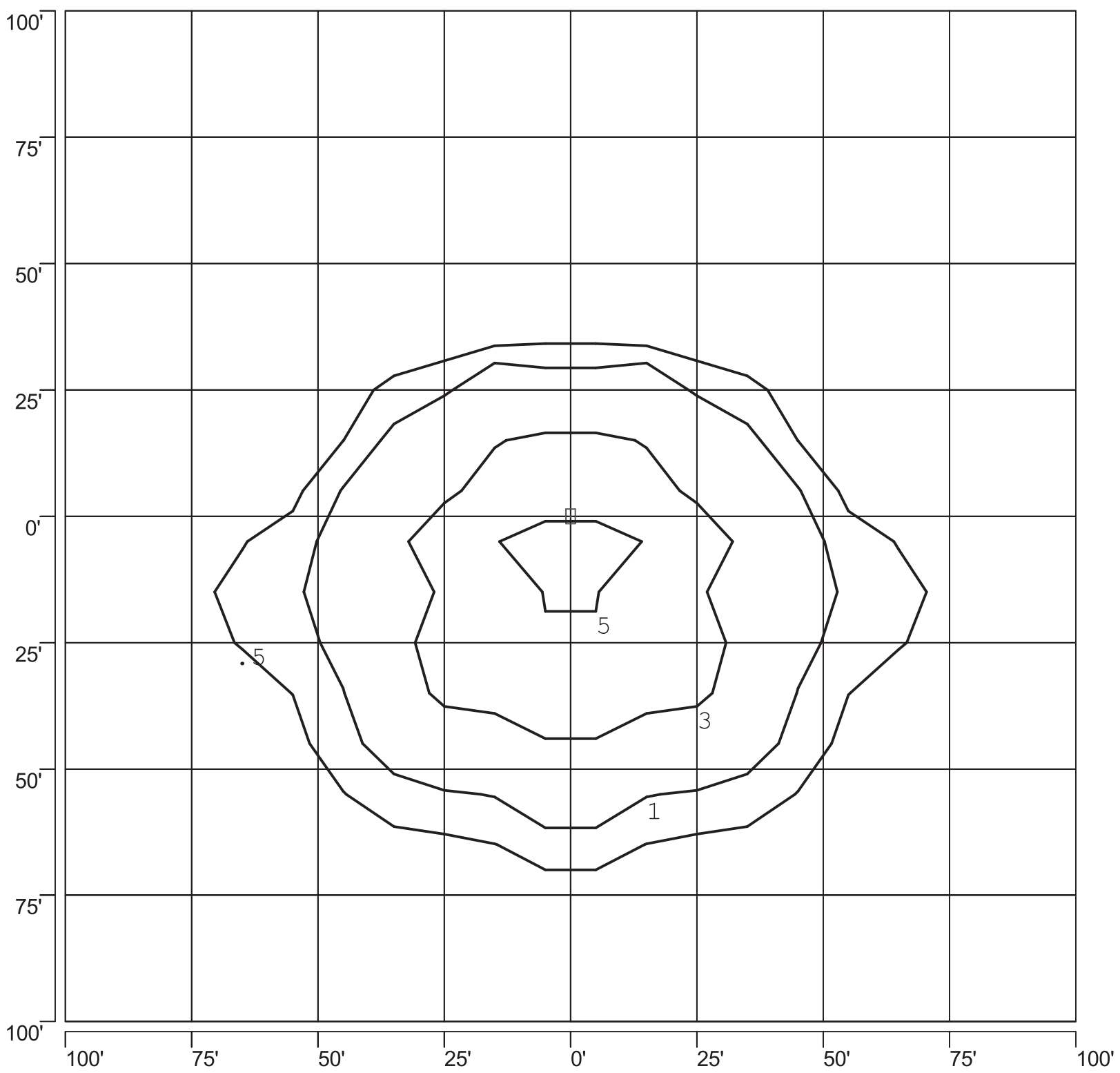
ISOFOOTCANDLE PLOT: VBMAJ3B_2-PS 400W PSMH TYPE III 25' AFG - 0 DEGREE TILT
