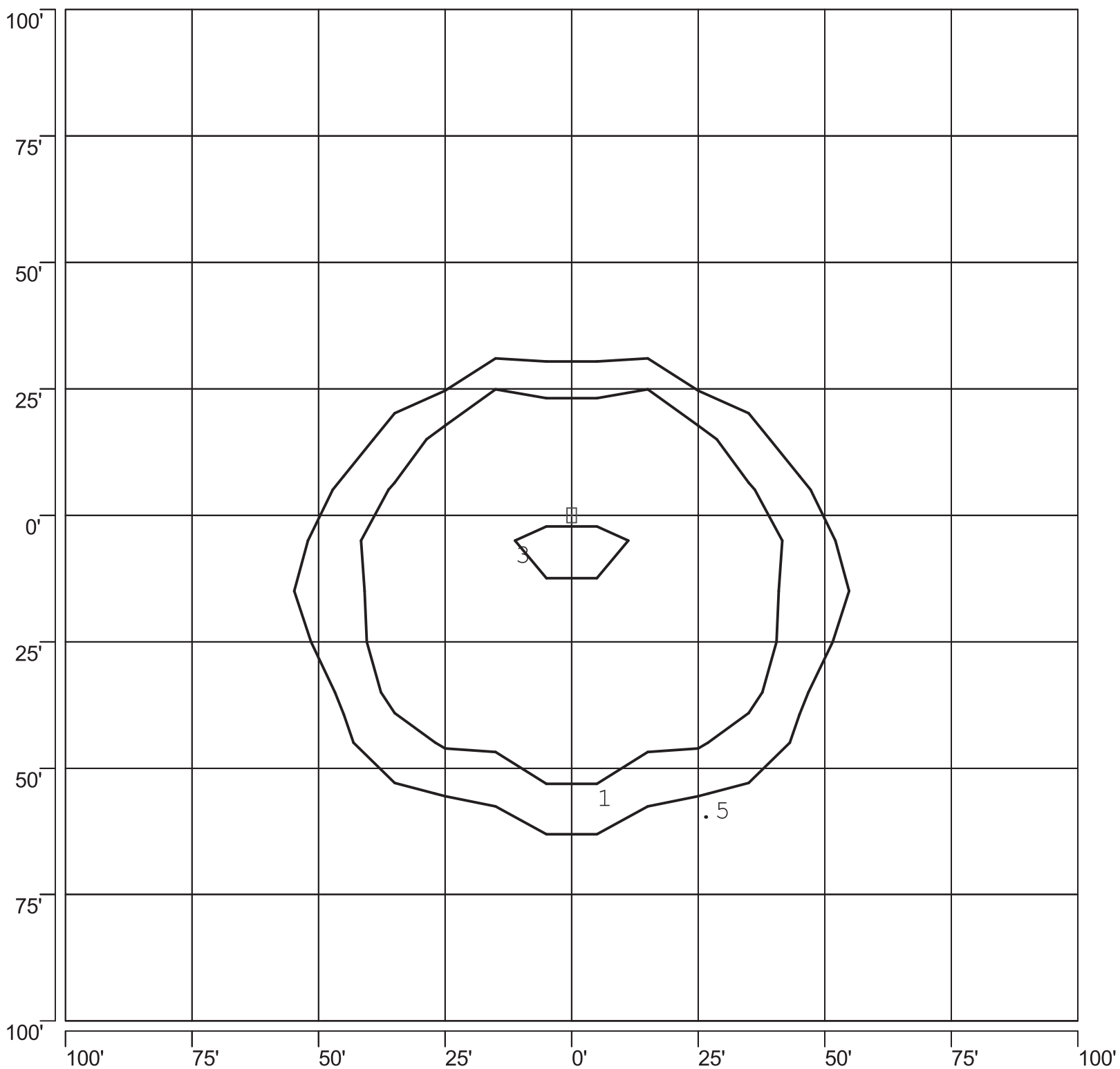
ISOFOOTCANDLE PLOT: VBMAJ1B_2-PS 250W PSMH TYPE III 25' AFG - 0 DEGREE TILT
