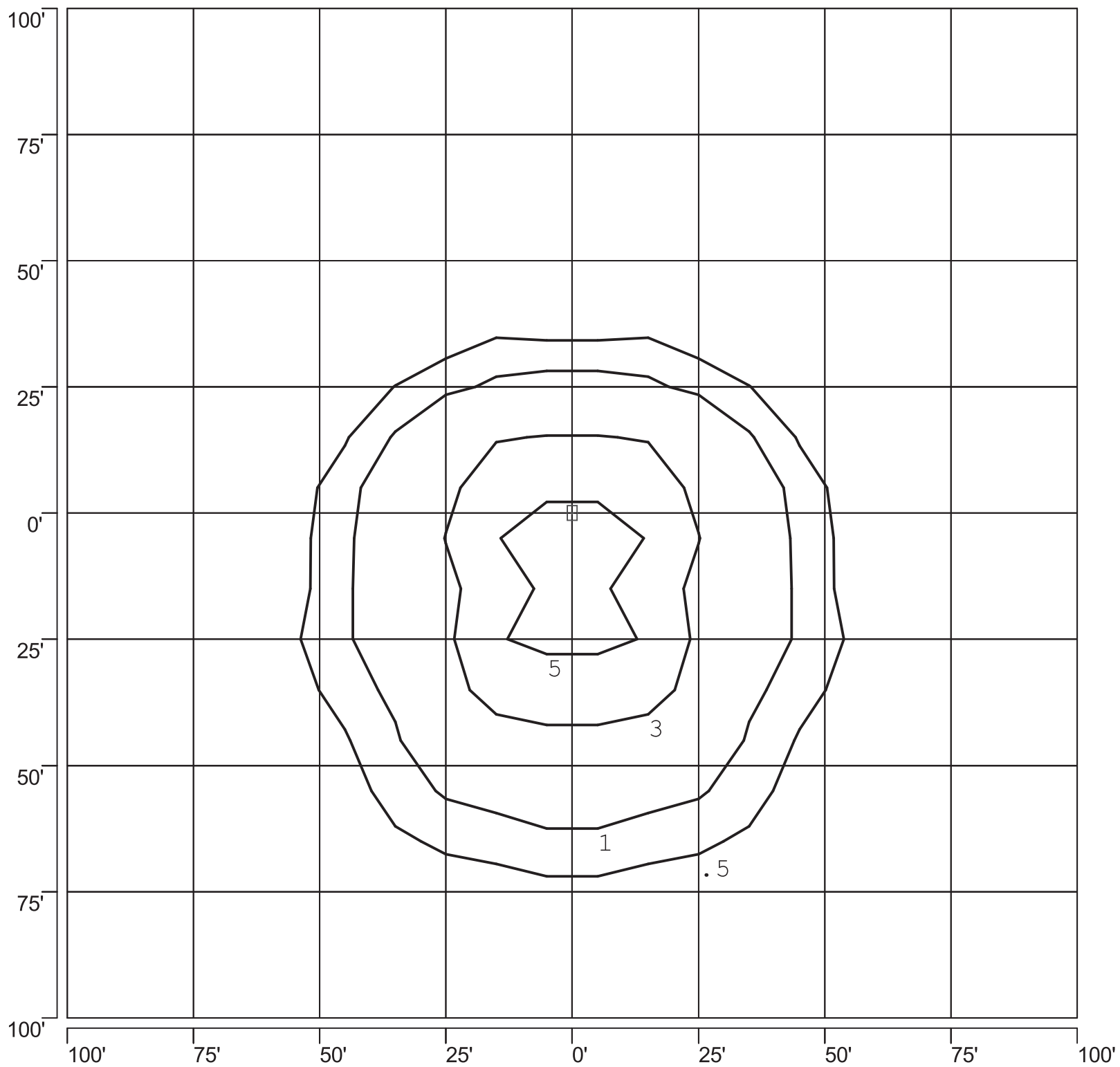
ISOFOOTCANDLE PLOT: VBMAG3B_2-PS 400W PSMH TYPE IV 25' AFG - 0 DEGREE TILT
